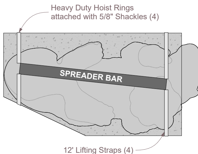
Pick Diagram - Plan
