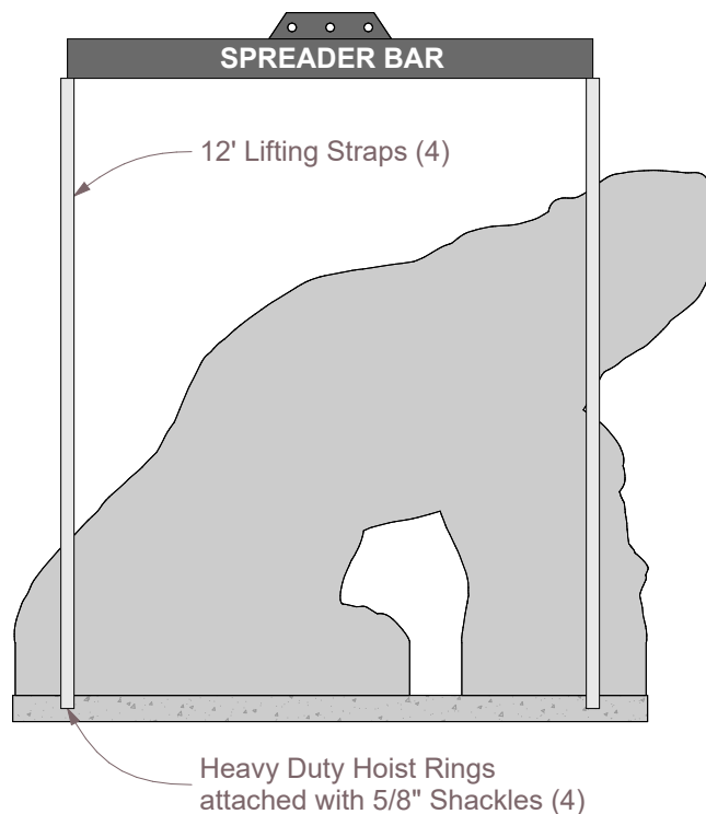
Pick Diagram - Elevation
